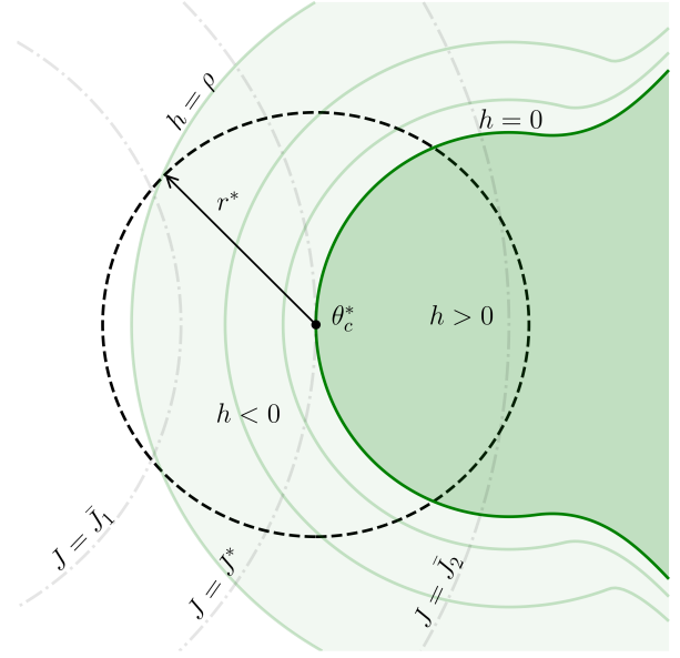
Fig. 2. Depiction of sets and levels of h and J with \bar{J}_1 < J^* < \bar{J}_2 . The safe set \mathcal{C} is shaded in dark green, which is contained by the set \mathcal{C}_\rho defined by both dark and light green shading. The radius r^* relates to the “angle condition” given in Assumption 4.
