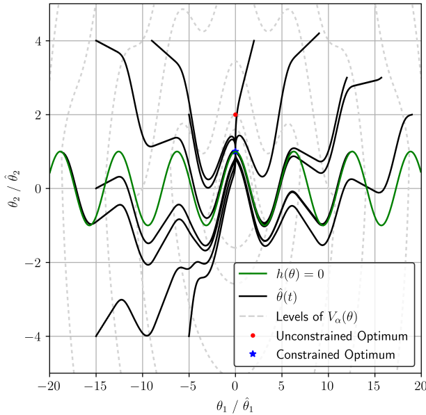
Fig. 4. Trajectories \hat{\theta} along with the safe boundary h(\theta) = 0 and level sets of V_\alpha with \alpha = 20 . The safe set is below the curve h(\theta) = 0 .
